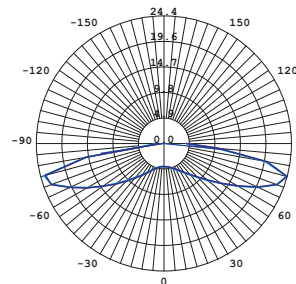
Scattering angle: 165°
